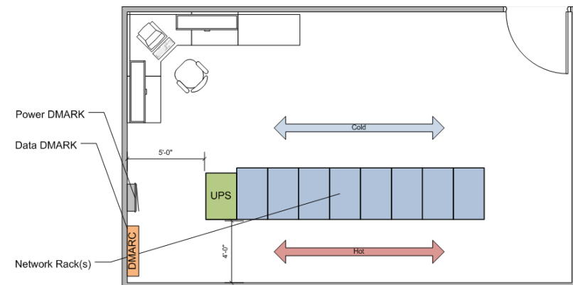
Data Suite - 500 sq. ft.
