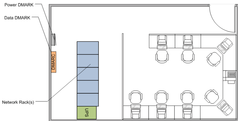
Data Suite - 500 sq. ft.
